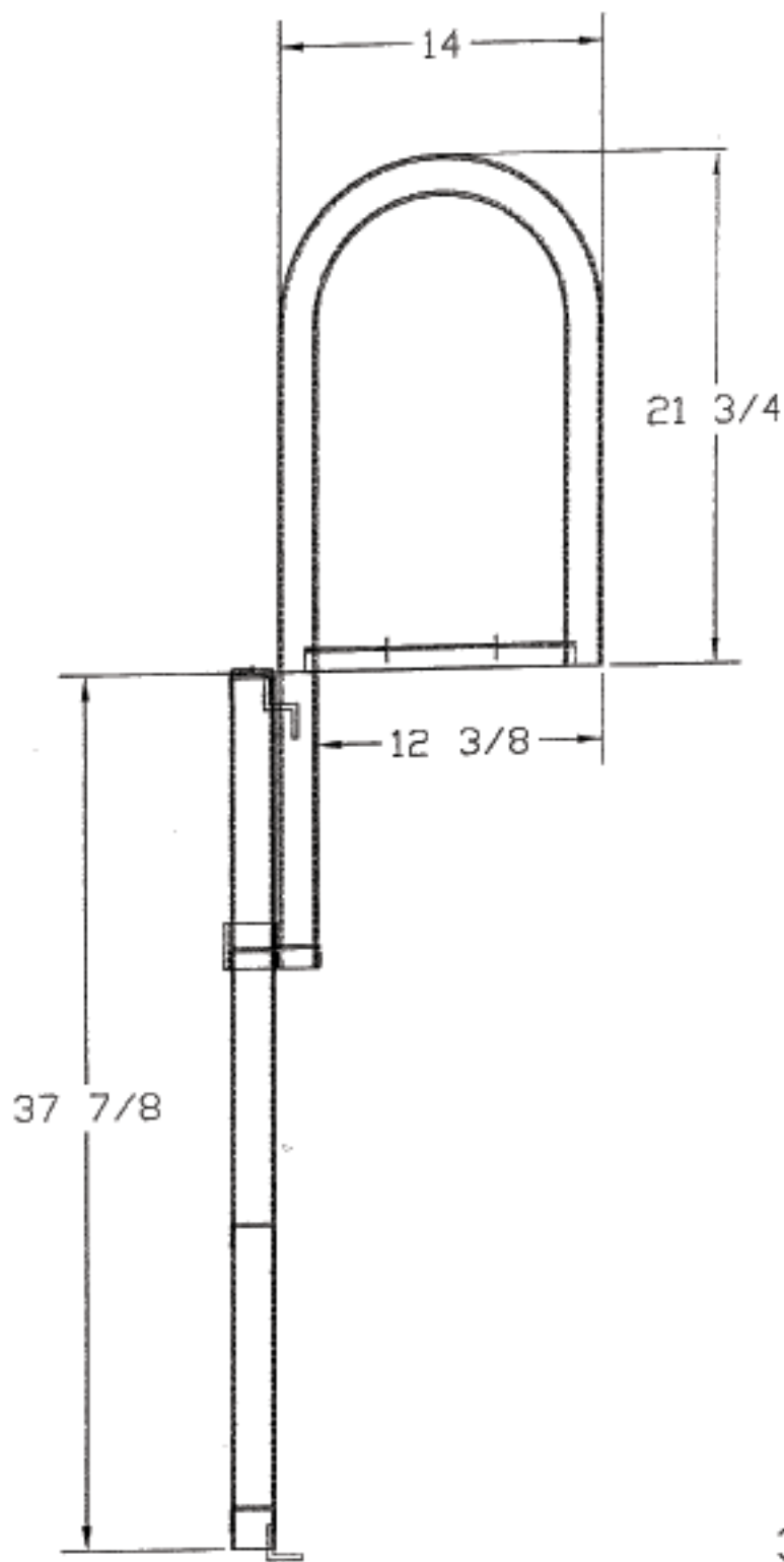
LADDER DOWN
